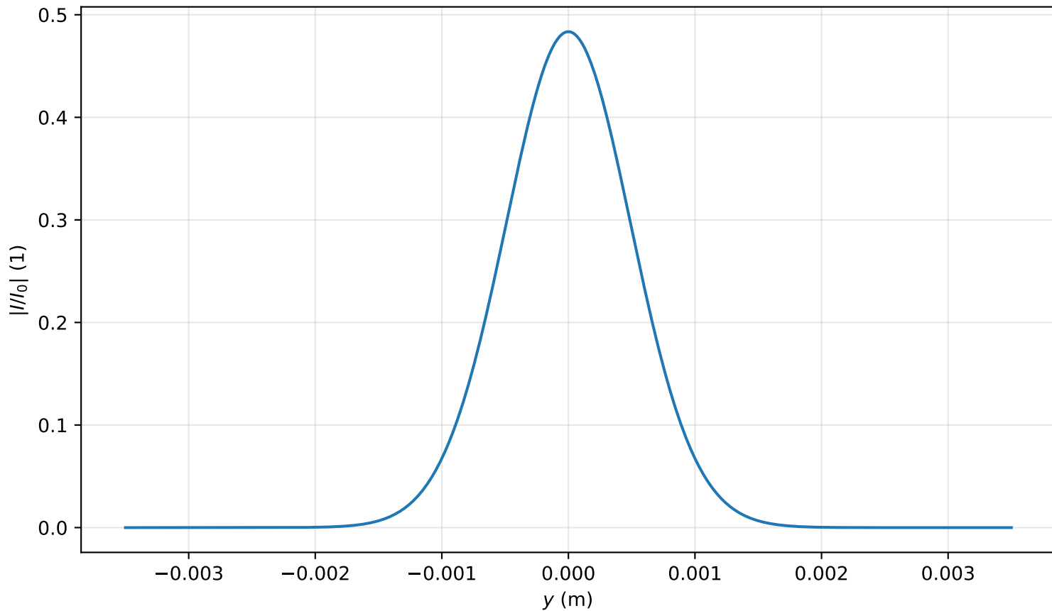
Intensity profile I(x = 0, y, z = 2.229)/I_0 , P_{in}=0.1P_{cr} , artificial time
